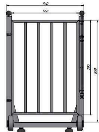
KPZ 2AV, 1510x560x850, 300 kg, division 100g, hot dip galvanized
