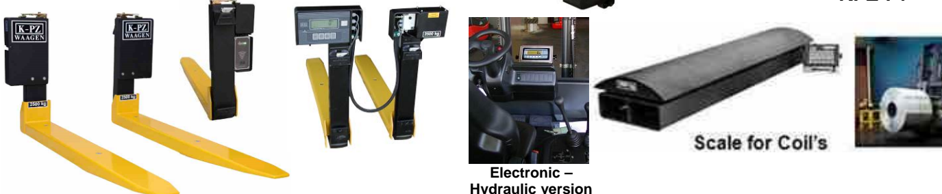
Weighing forks Forklift truck scale
